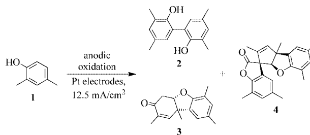
Scheme 1. Oxidative coupling reaction of 1 .
