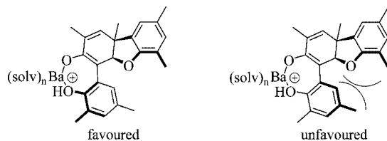
Figure 2. Possible conformations of intermediate 4b in methanolic barium hydroxide.
