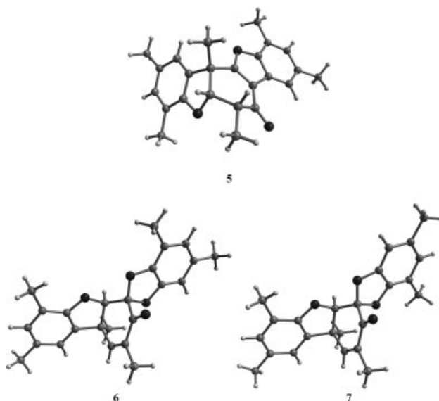
Figure 4. X-ray structure of pentacycles 5 , 6 , and 7 .
