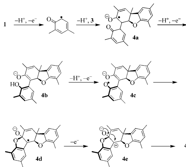
Scheme 2. Proposed mechanism for the formation of pentacyclic spiro lactone 4 .
