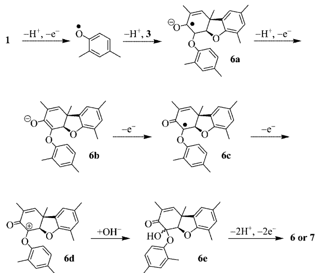
Scheme 3. Proposed mechanism for the formation of benzodioxoles 5 and 6 .
