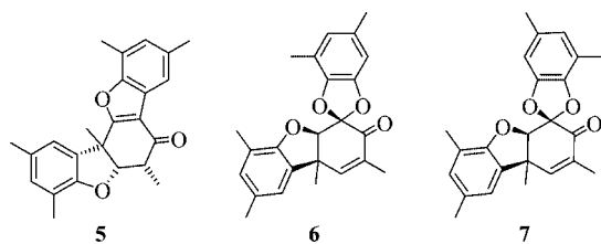
Figure 3. Oxidatively-coupled trimers of 1 .
