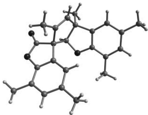
Figure 1. X-ray structure of pentacyclic spiro lactone 4 .
